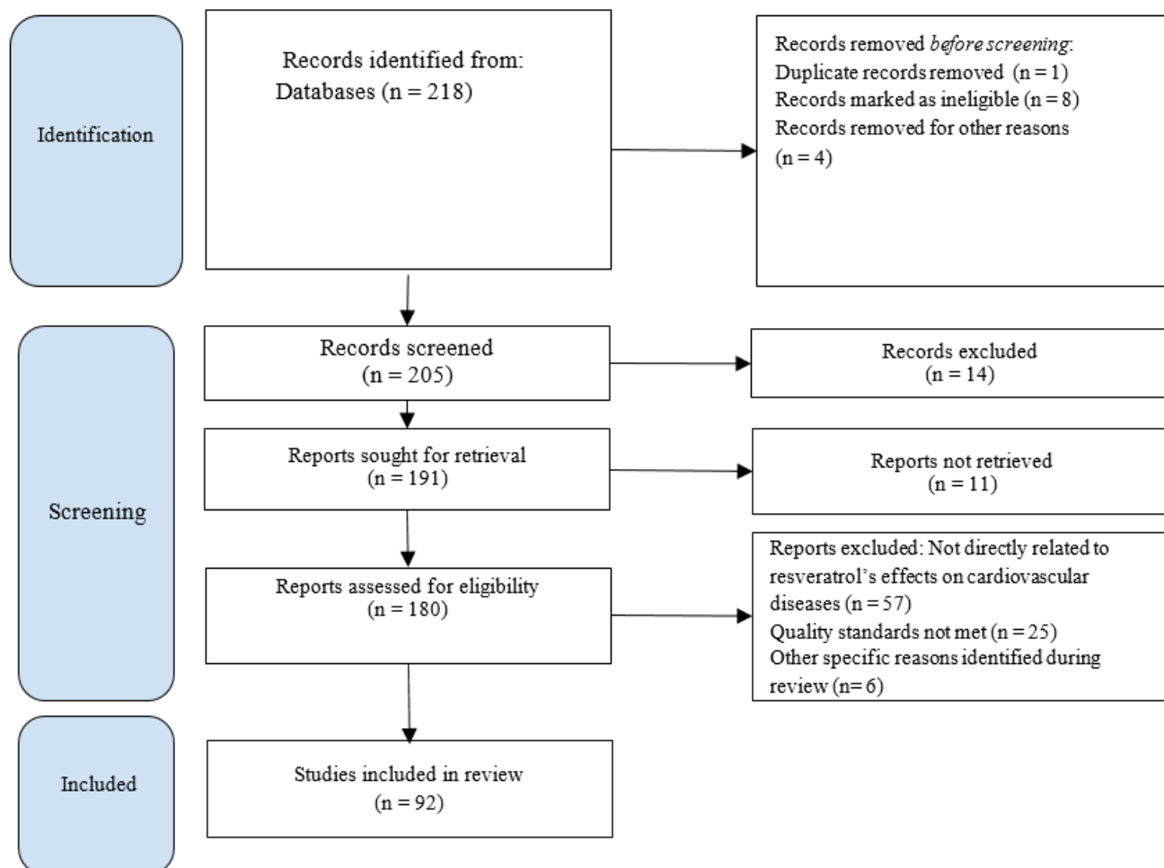
Study selection flow chart
