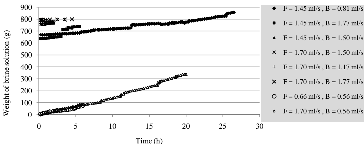
Fig. 2. Changes in stripping solution weight during the concentration of initial red beet juice (without clarification) using osmotic distillation (F = Juice flow rate, B = Brine flow rate).
