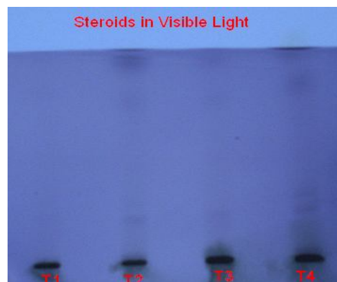
Fig.1. HPTLC analysis of steroids. Steroids after derivatisation with 5% sulphuric acid
